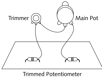
FIGURE A-8: Don't be surprised if you find a cool spot for a potentiometer to either adjust pitch or to vary some other interesting effect, only to discover that when turned all the way down (presenting no resistance to the circuit) the circuit quickly crashes. What's needed is to ensure that there's still a little resistance left in the bend when the pot's turned all the way down—to zero resistance. As shown in the diagram, the answer is simple: Once the trimmer is installed in line with the main potentiometer, all that's left is to set the trimmer to the resistance needed to keep the circuit from "seeing" zero resistance and crashing when the pot is turned all the way down. Turn the trimmer up all the way; turn the main pot down. With the bend running, turn the trimmer down until just pre-crash. This sets a safe operational minimum resistance for the bend.
